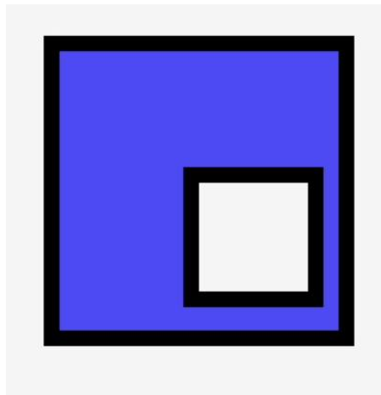
Subtract Selection
