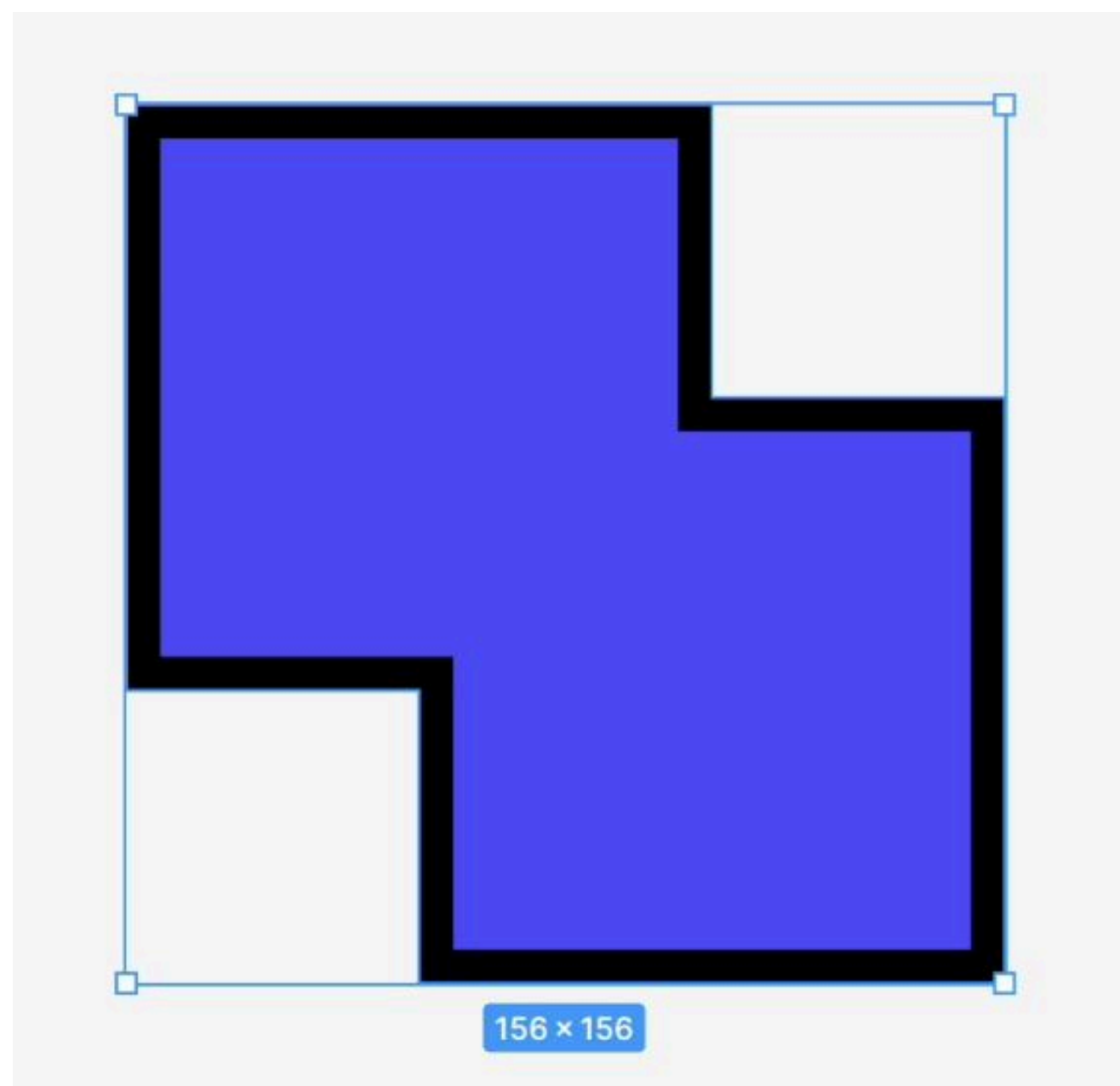
Union Selection
