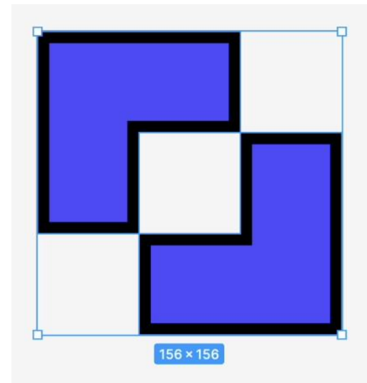
Exclude Selection
